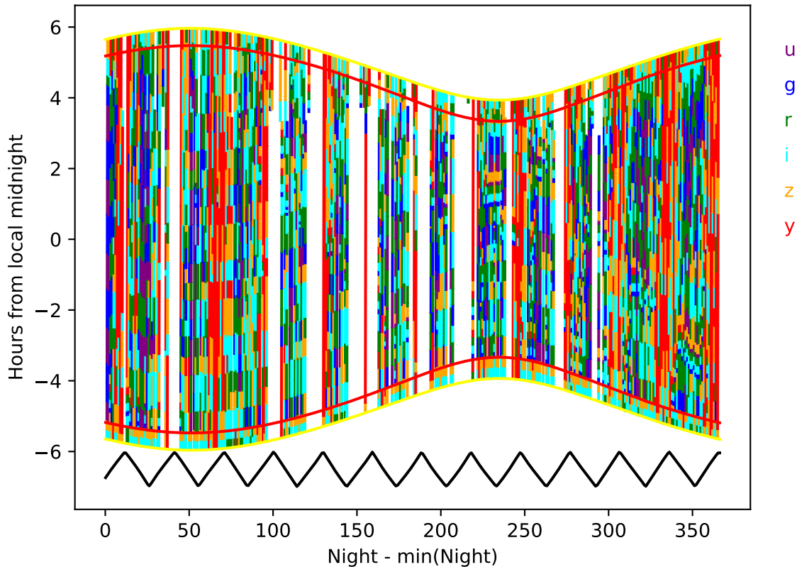
weather_cloudso30v3.4_10yrs year 0-1: Hourglass
