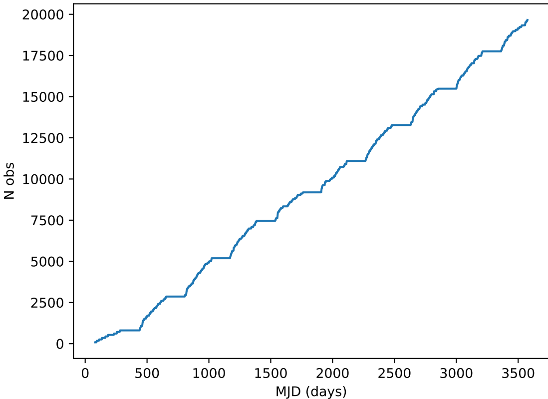
weather_cloudso30v3.4_10yrs note like DD:XMM_LSS%: Cumulative
