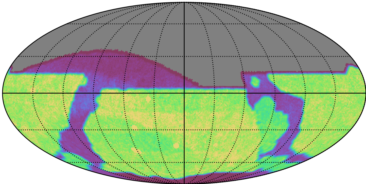
weather_cloudso30v3.4_10yrs z: Count observationStartMJD
