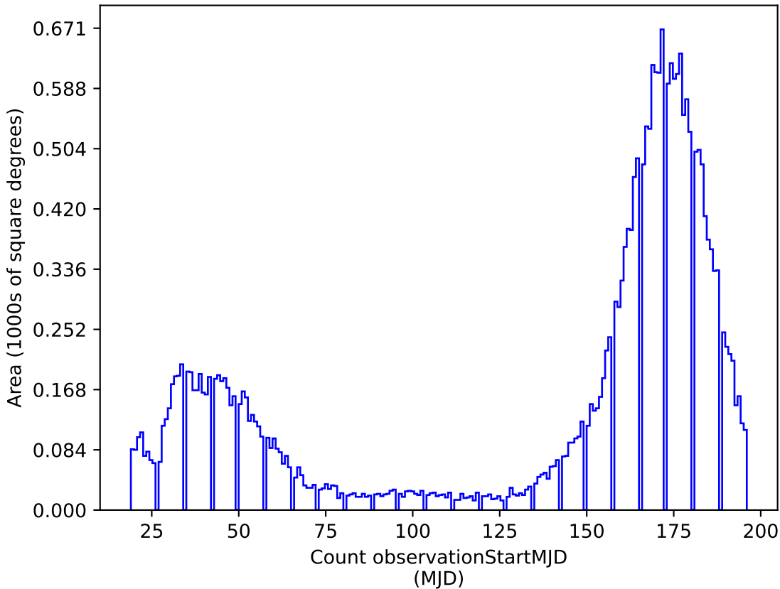
weather_cloudso30v3.4_10yrs z: Count observationStartMJD
