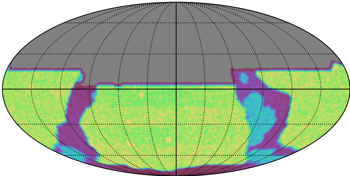
weather_cloudso30v3.4_10yrs y: Count observationStartMJD
