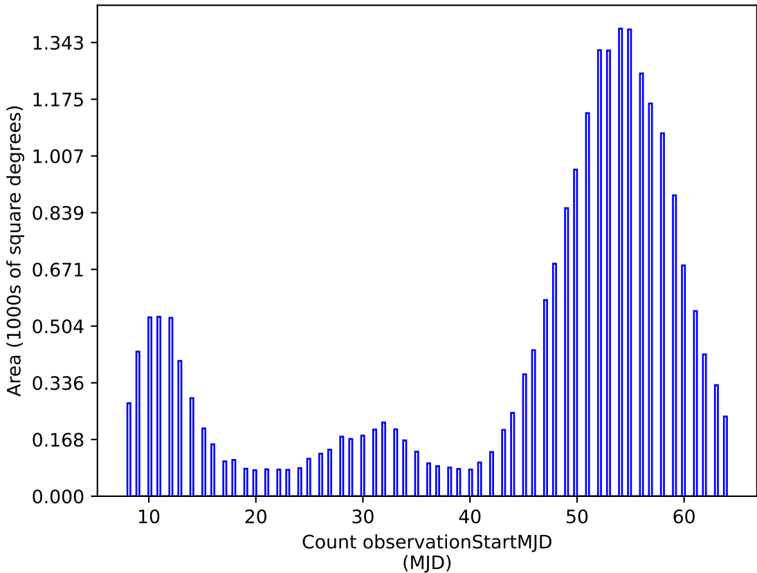
weather_cloudso30v3.4_10yrs u: Count observationStartMJD
