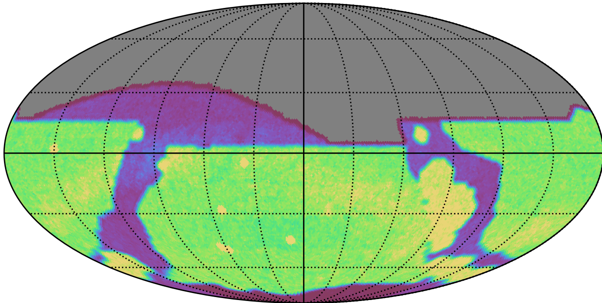
weather_cloudso30v3.4_10yrs r: Count observationStartMJD
