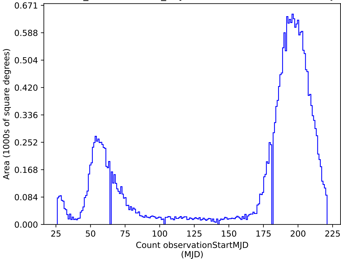
weather_cloudso30v3.4_10yrs i: Count observationStartMJD
