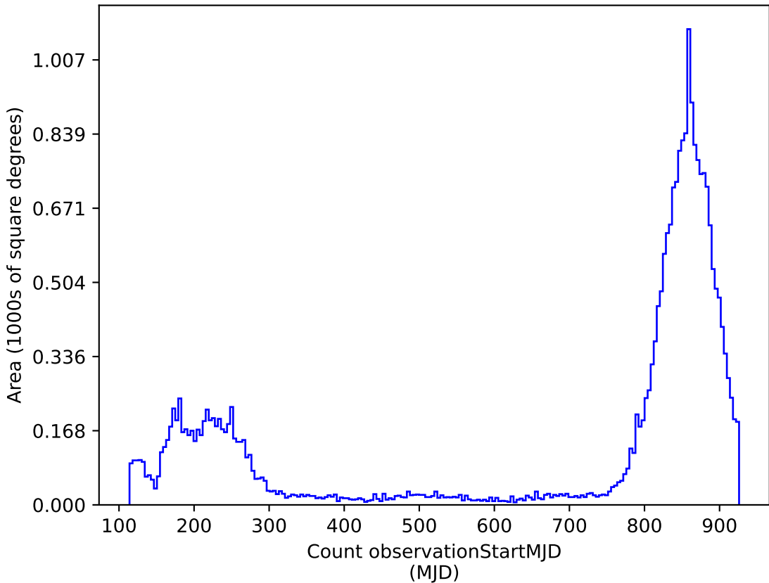
weather_cloudso30v3.4_10yrs : Count observationStartMJD
