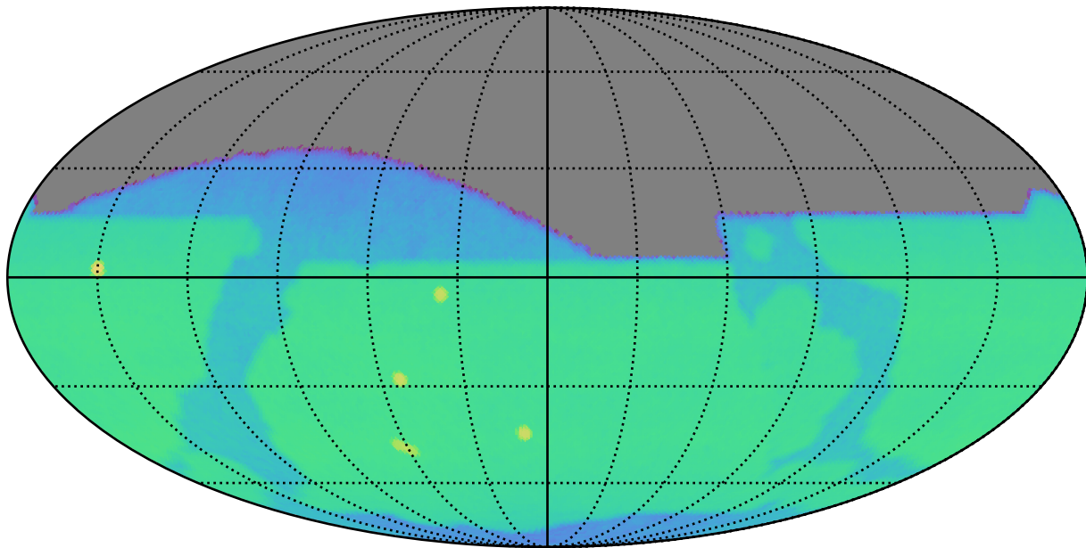
weather_cloudso30v3.4_10yrs z: CoaddM5
