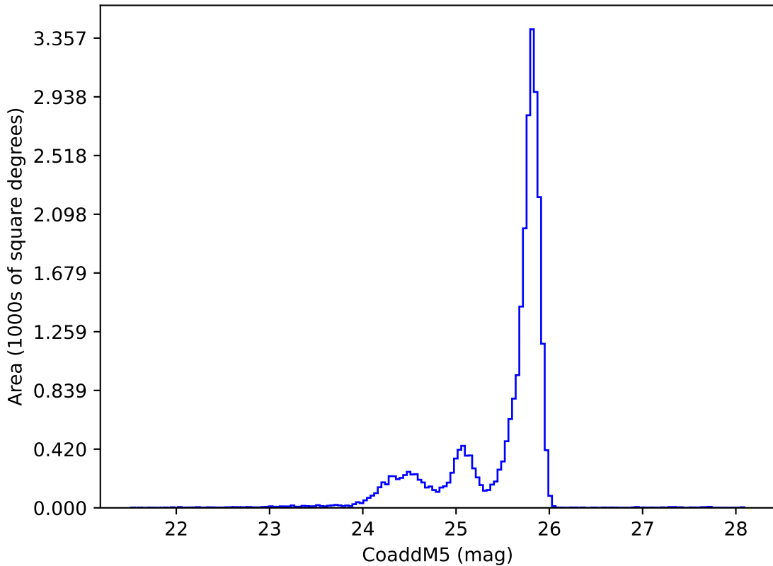
weather_cloudso30v3.4_10yrs z: CoaddM5
