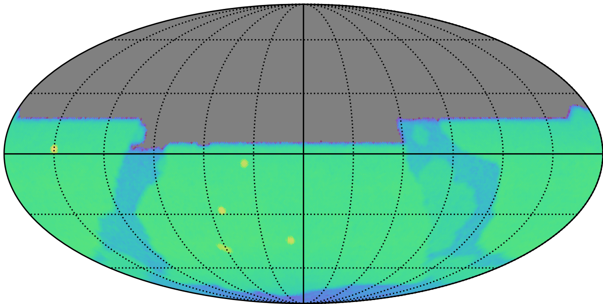
weather_cloudso30v3.4_10yrs y: CoaddM5
