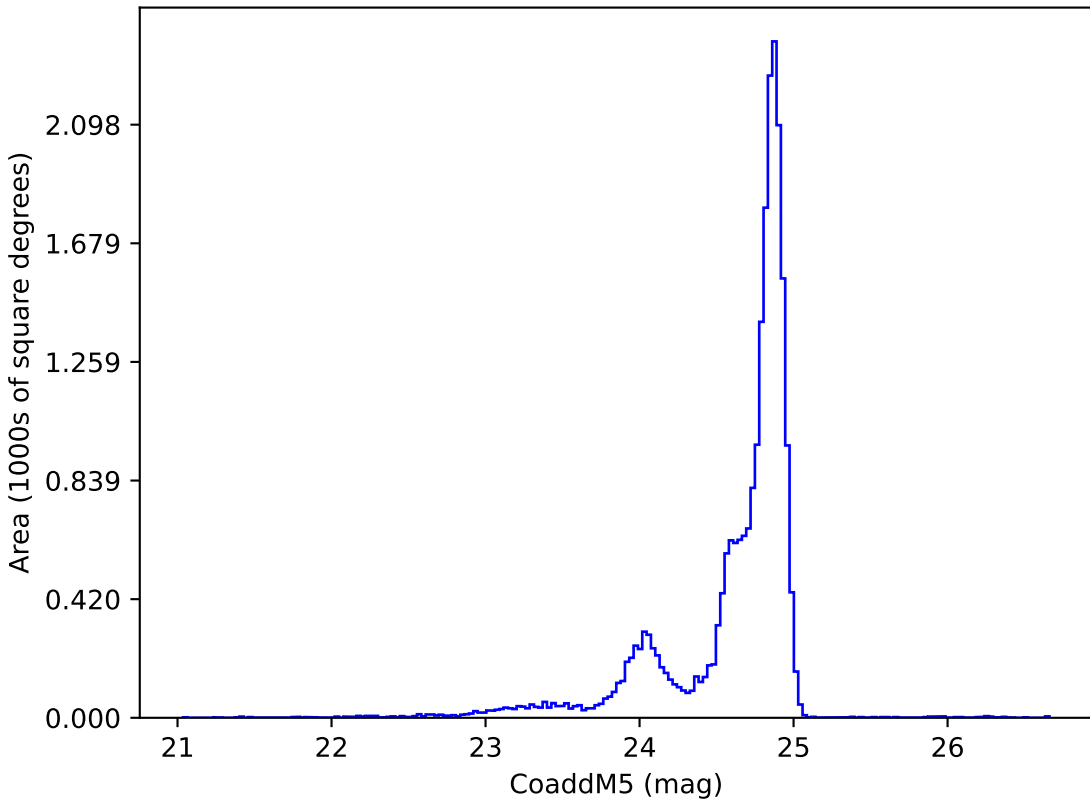
weather_cloudso30v3.4_10yrs y: CoaddM5
