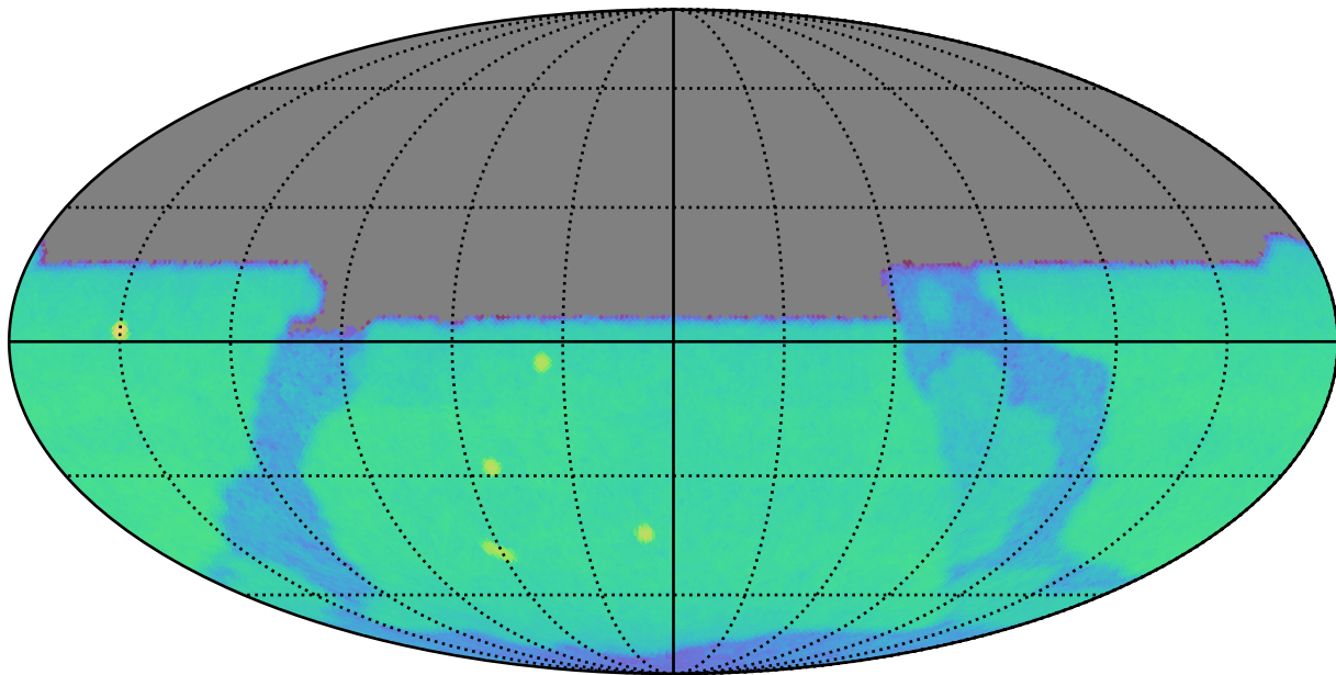
weather_cloudso30v3.4_10yrs u: CoaddM5
