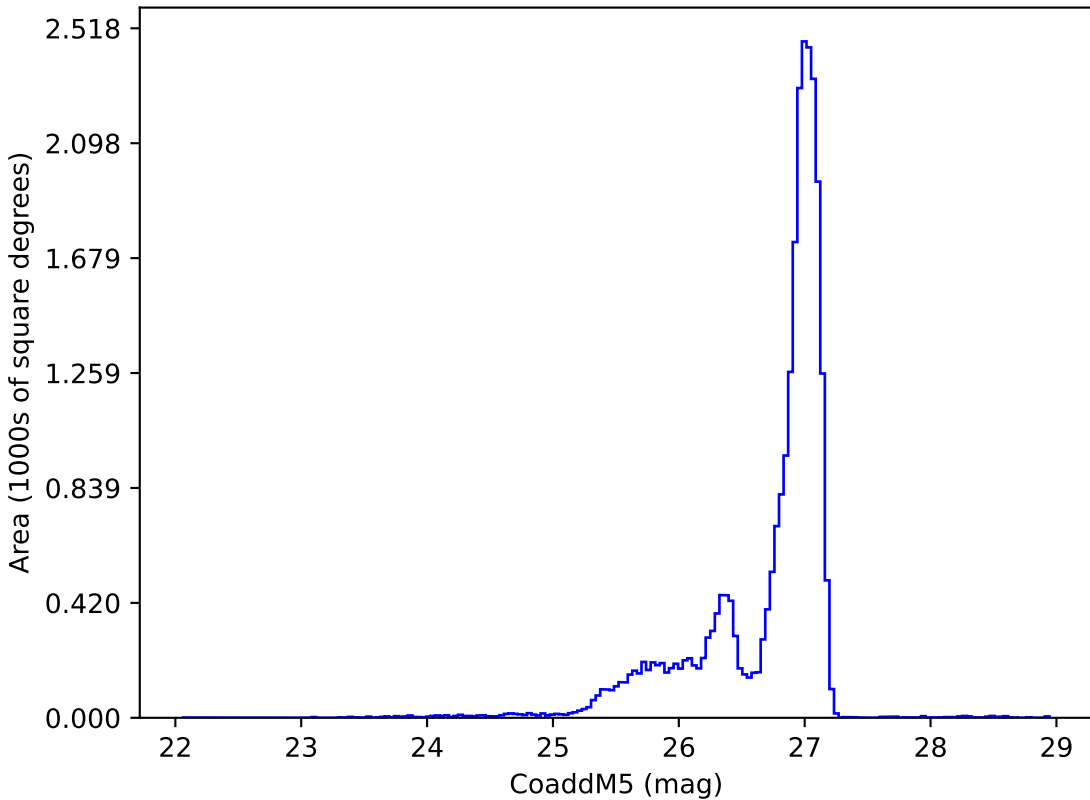
weather_cloudso30v3.4_10yrs r: CoaddM5
