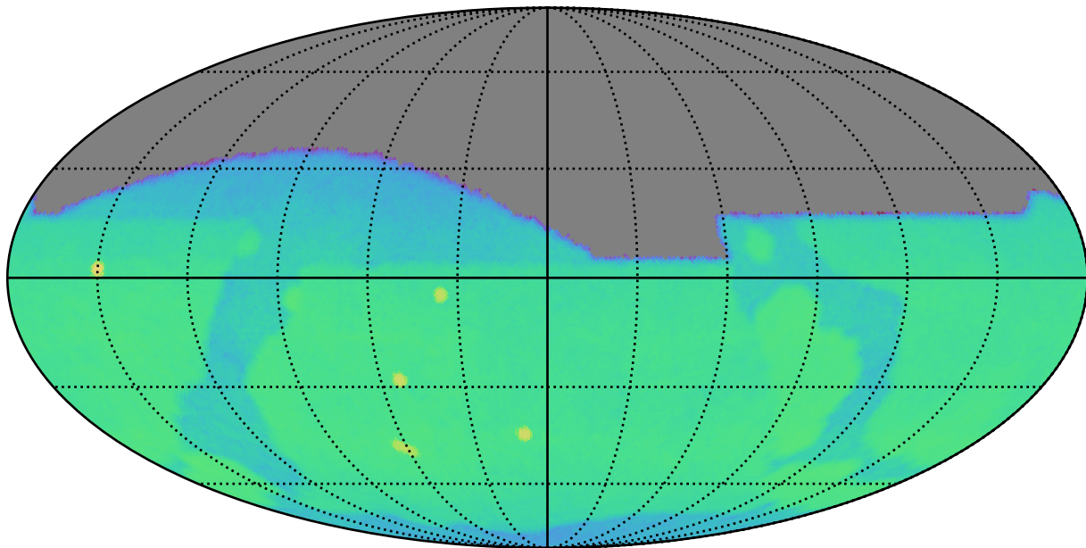
weather_cloudso30v3.4_10yrs g: CoaddM5
