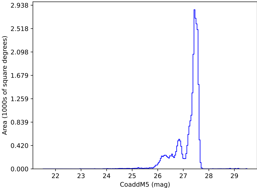
weather_cloudso30v3.4_10yrs : CoaddM5
