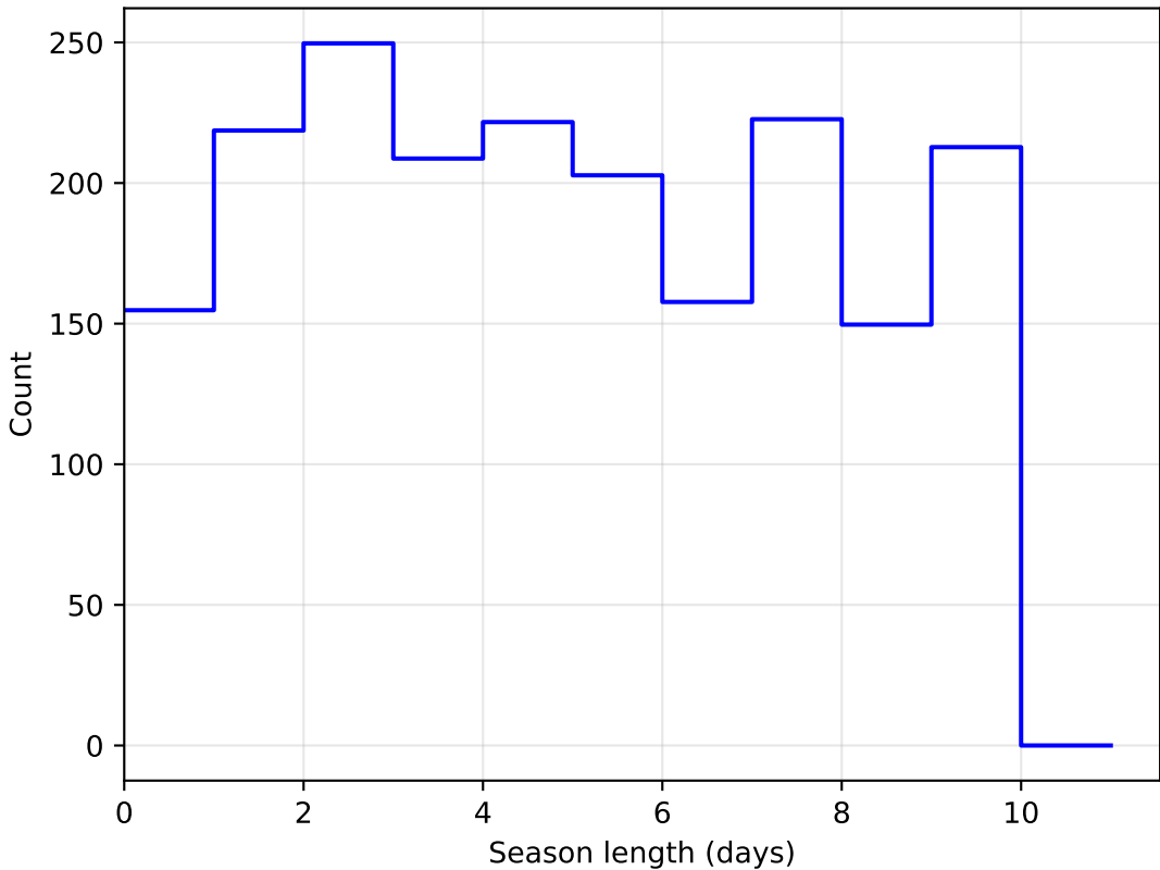
weather_cloudso30v3.4_10yrs DD:WFD all bands: SeasonLength
