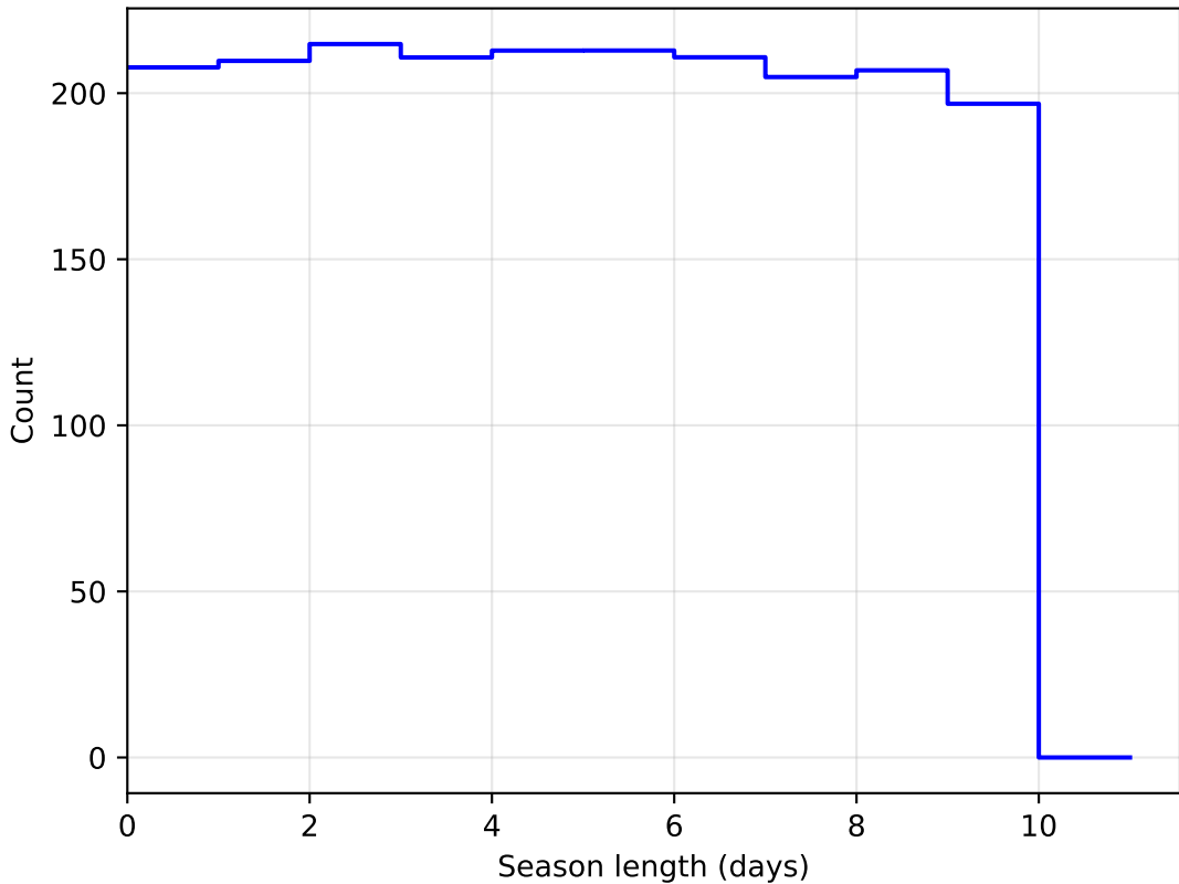
weather_cloudso30v3.4_10yrs DD:EDFS all bands: SeasonLength
