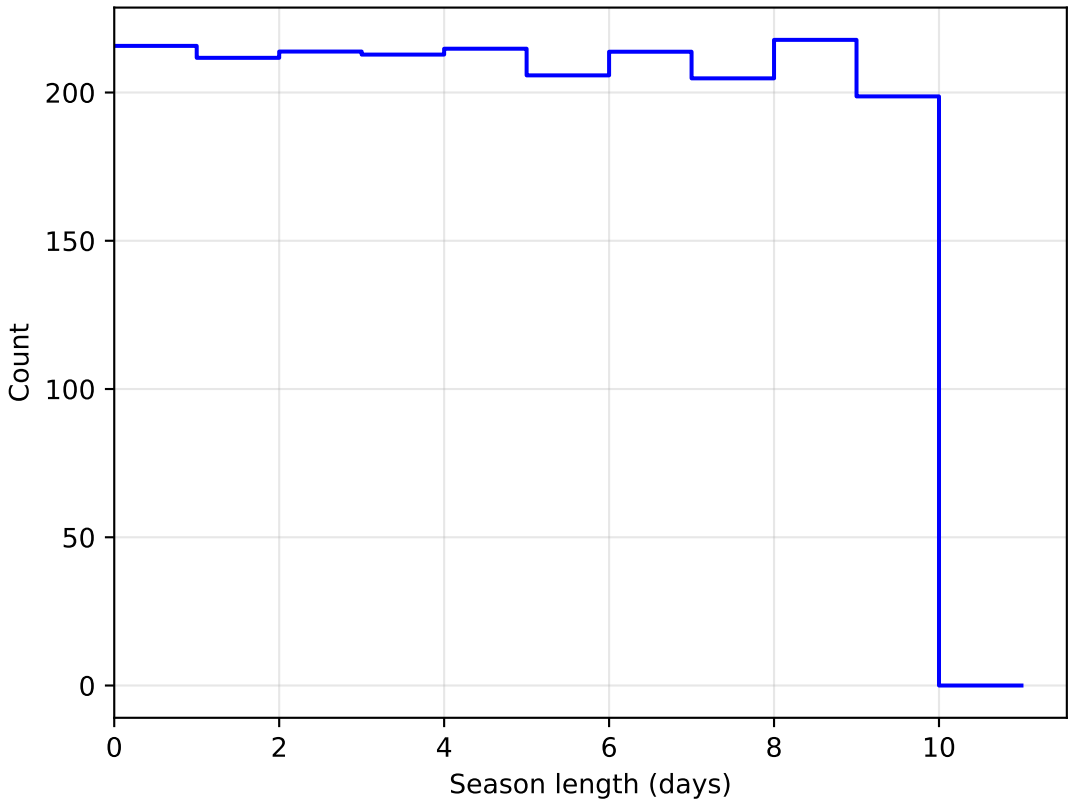
weather_cloudso30v3.4_10yrs DD:ECDFS all bands: SeasonLength
