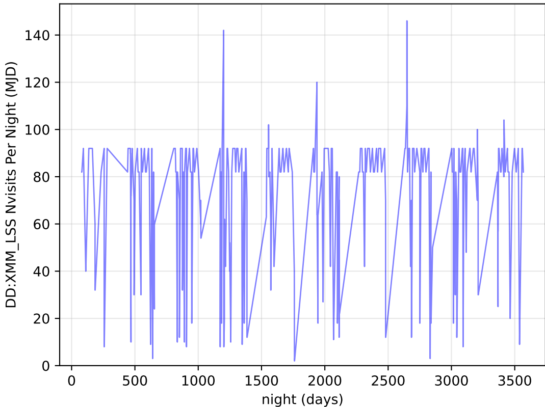
weather_cloudso30v3.4_10yrs all bands: DD:XMM_LSS Nvisits Per Night
