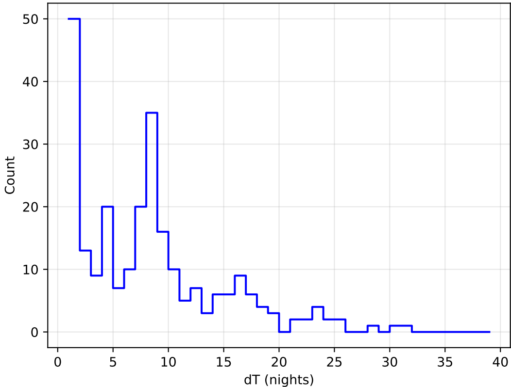
weather_cloudso30v3.4_10yrs all bands: DD:XMM_LSS Delta Nights Histogram
