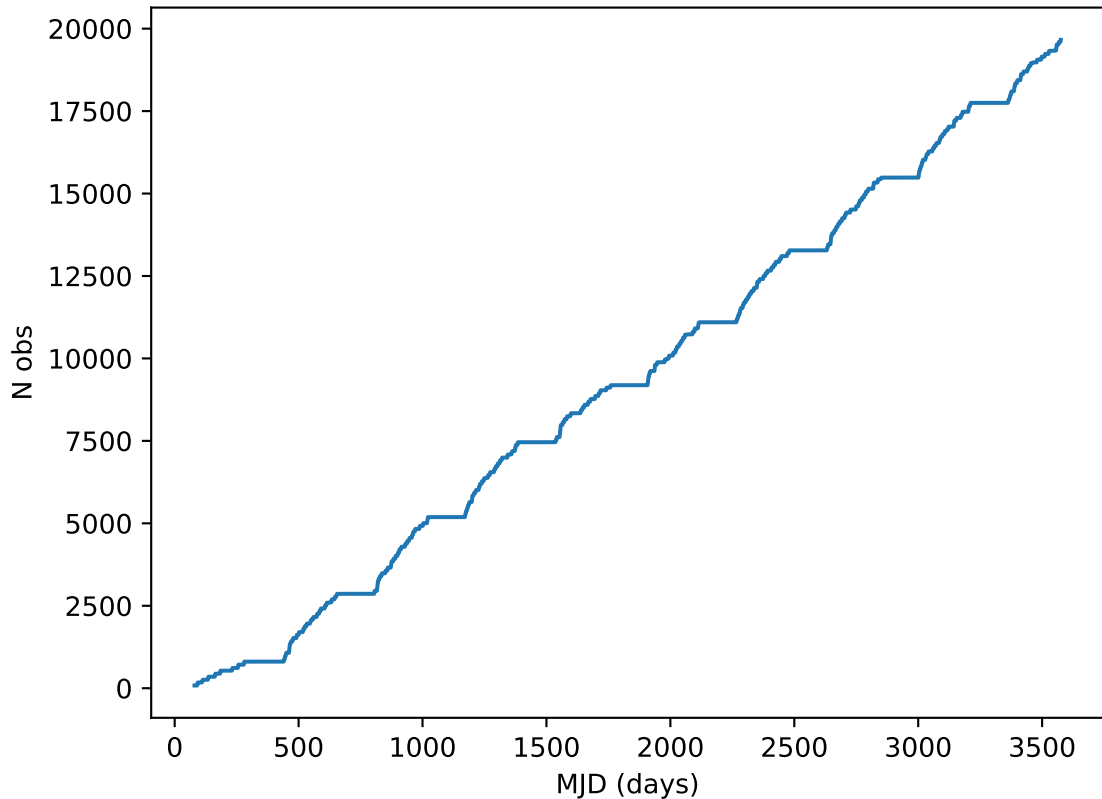
weather_cloudso30v3.4_10yrs all bands: DD:XMM_LSS Cumulative NVisits
