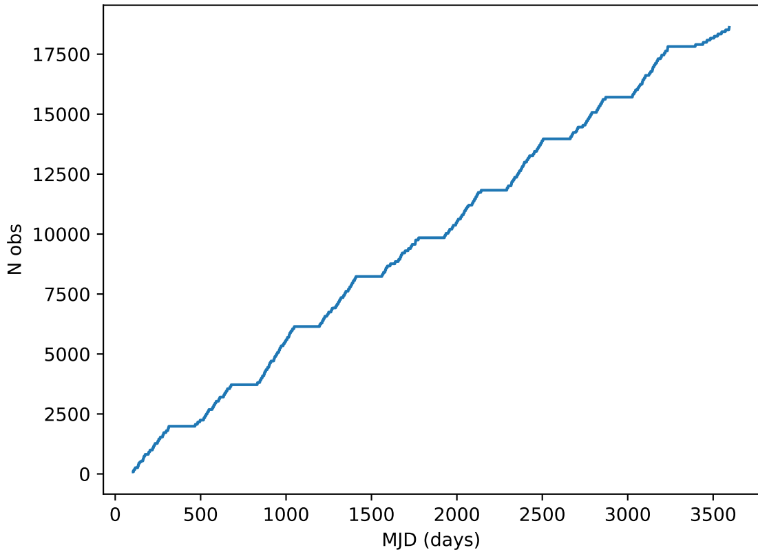
weather_cloudso30v3.4_10yrs all bands: DD:EDFS Cumulative NVisits
