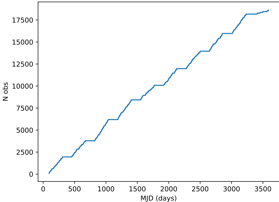
weather_cloudso30v3.4_10yrs all bands: DD:ECDFS Cumulative NVisits
