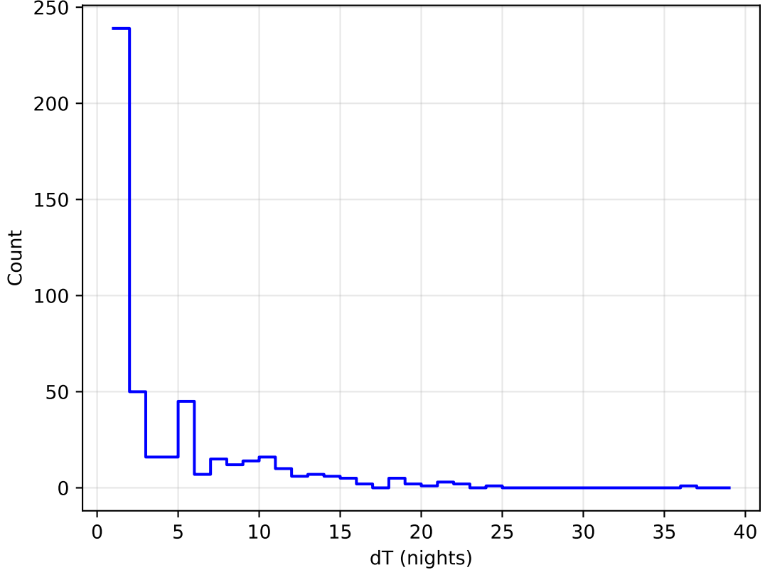
weather_cloudso30v3.4_10yrs all bands: DD: COSMOS Delta Nights Histogram
