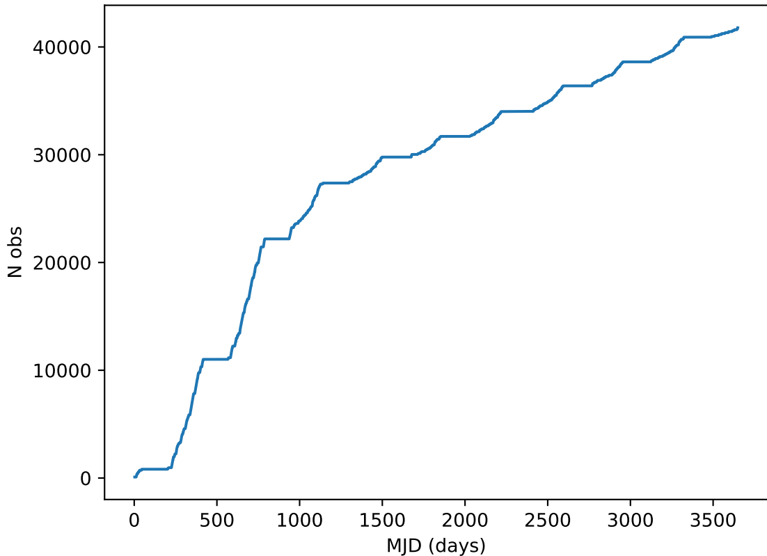
weather_cloudso30v3.4_10yrs all bands: DD:COSMOS Cumulative NVisits
