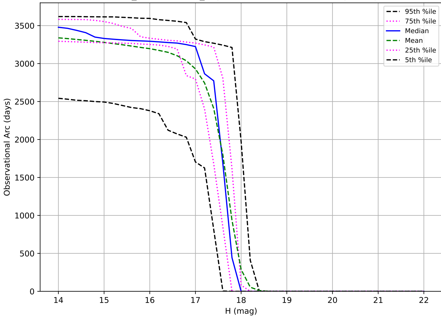
weather_cloudso2v3.4_10yrs: Observational Arc Length Trojan
