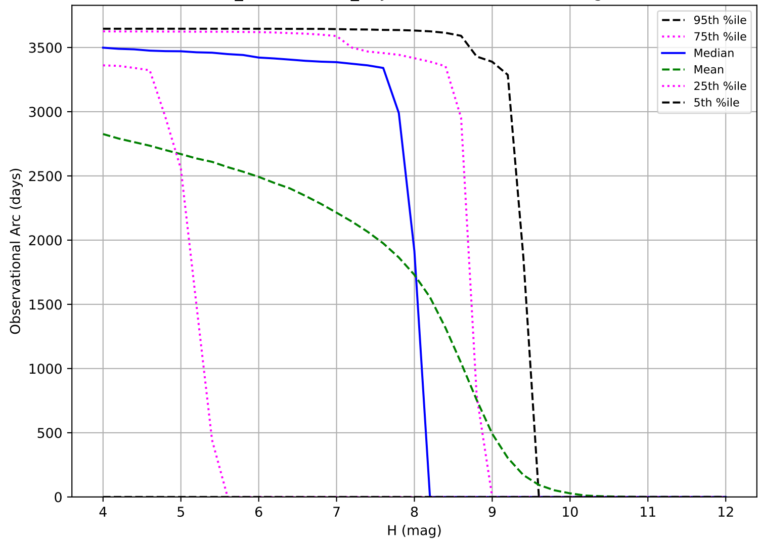
weather_cloudso2v3.4_10yrs: Observational Arc Length TNO
