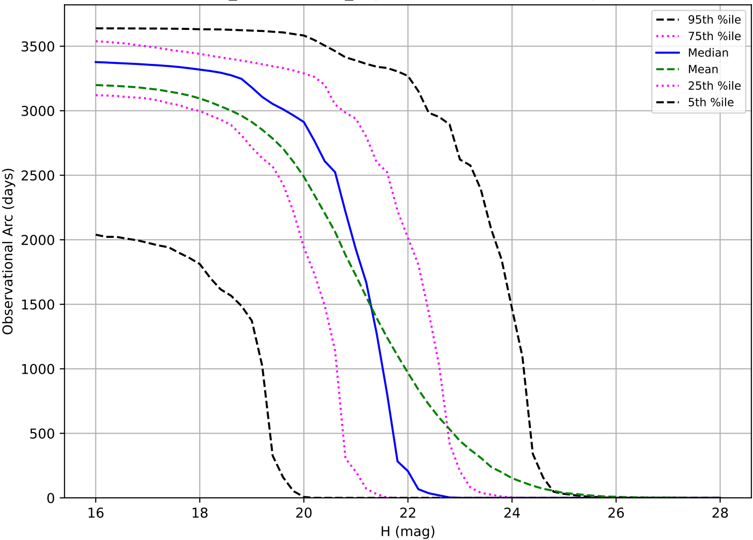
weather_cloudso2v3.4_10yrs: Observational Arc Length PHA
