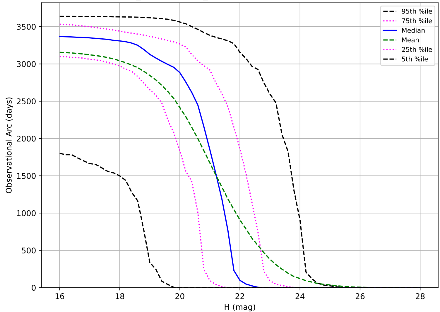
weather_cloudso2v3.4_10yrs: Observational Arc Length NEO
