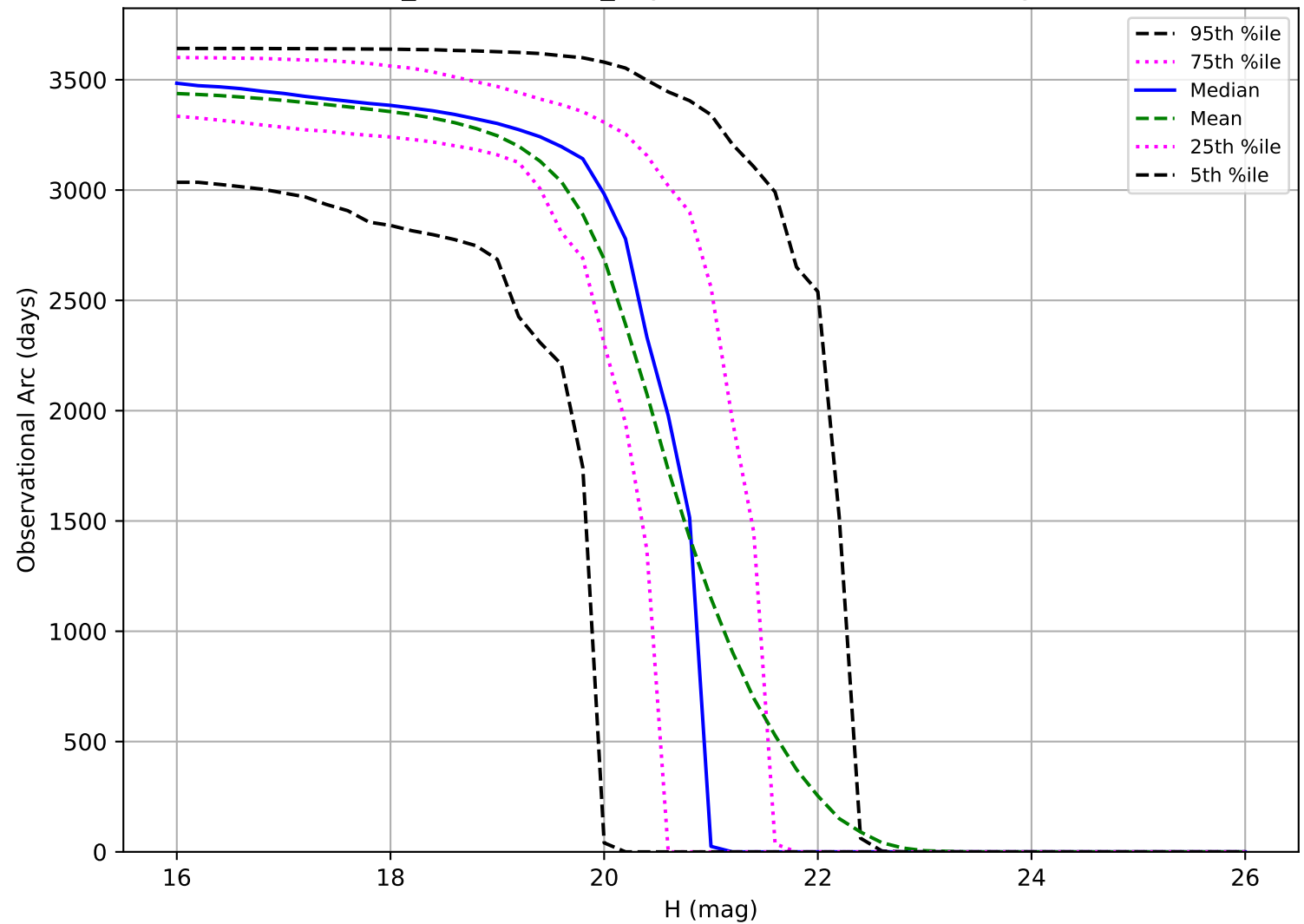
weather_cloudso2v3.4_10yrs: Observational Arc Length MBA
