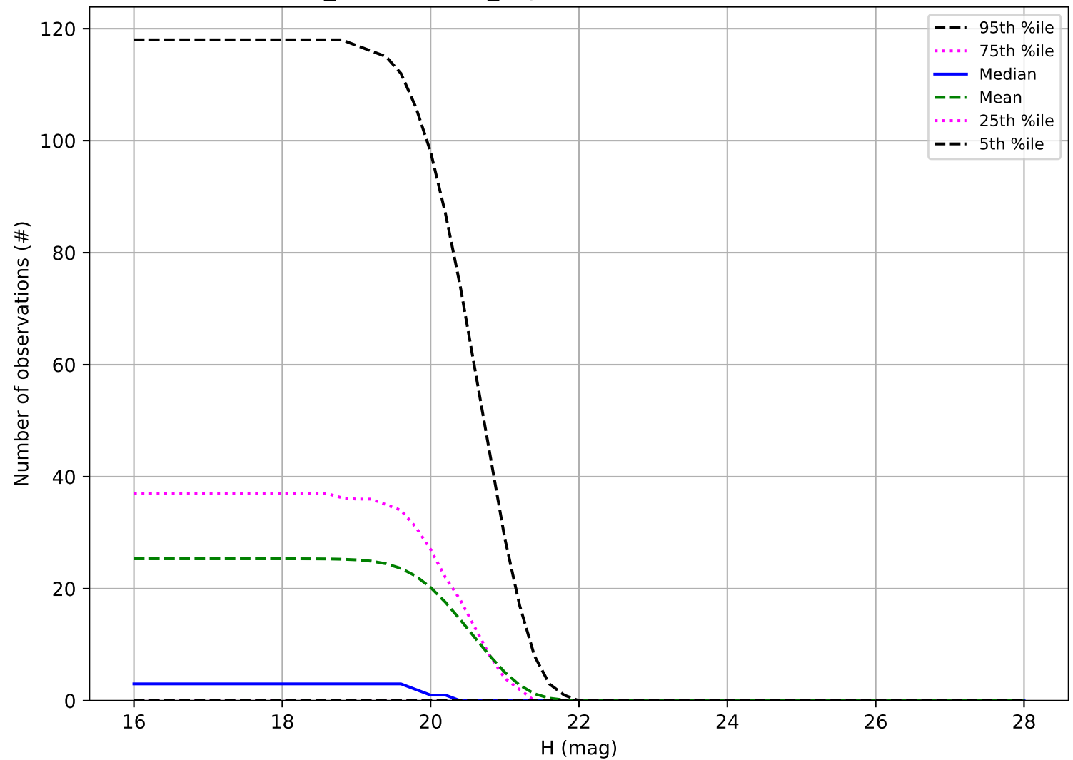
weather_cloudso2v3.4_10yrs: Number of observations Vatira
