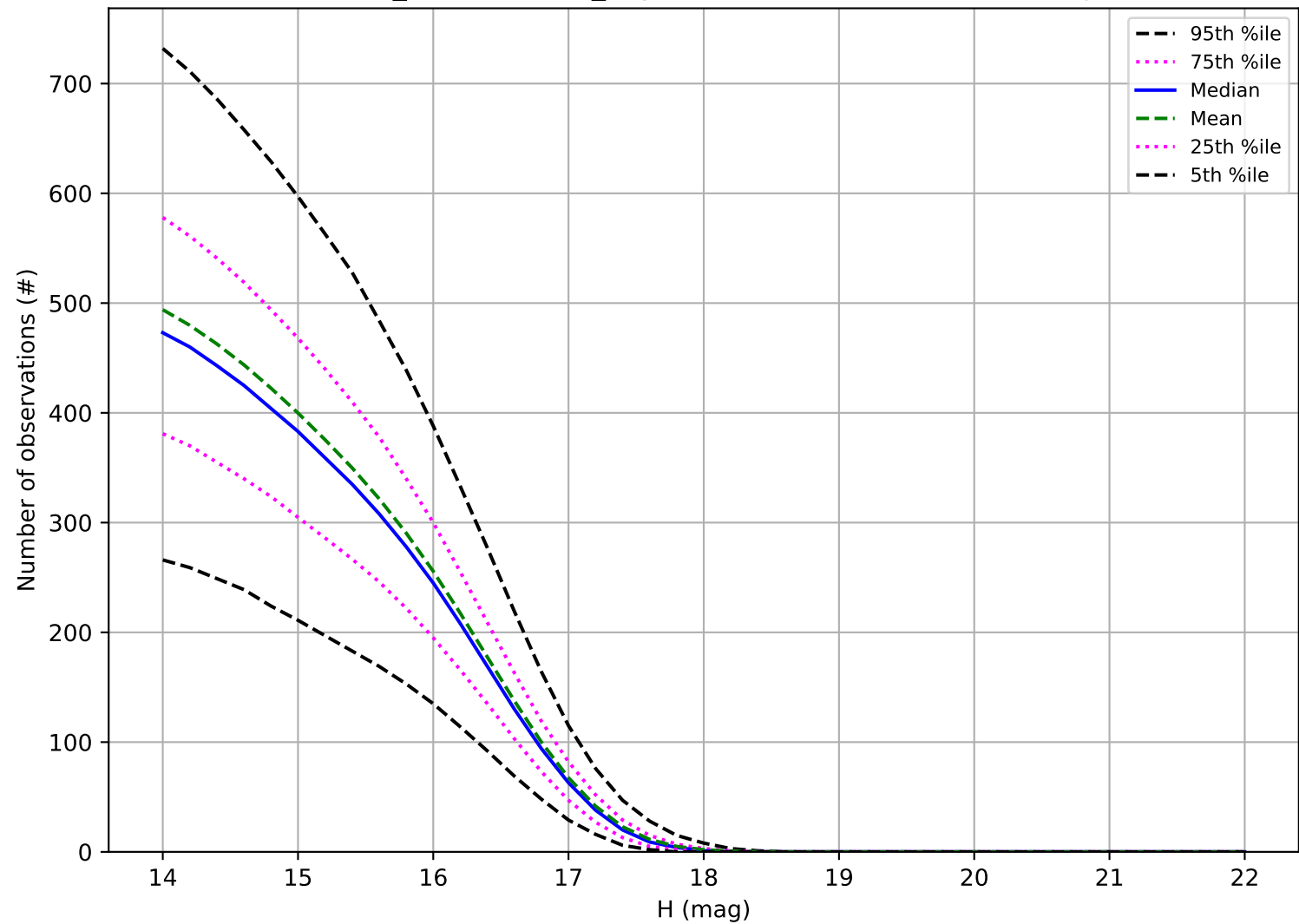
weather_cloudso2v3.4_10yrs: Number of observations Trojan
