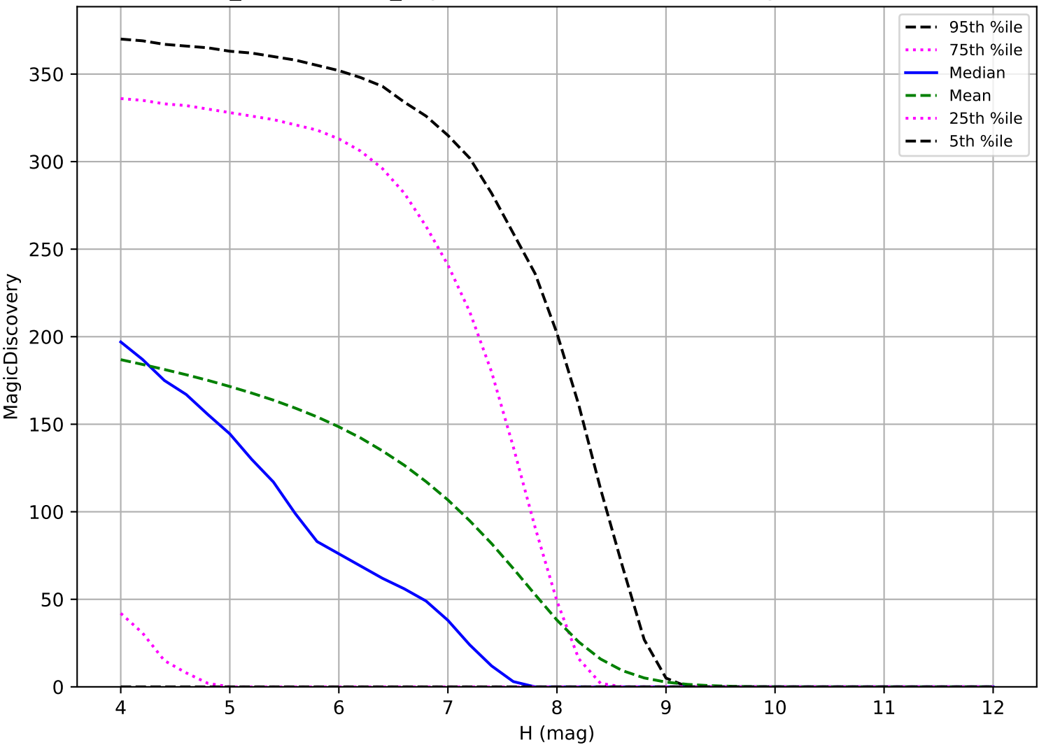
weather_cloudso2v3.4_10yrs: TNO 6 detections in 60 nights detection loss
