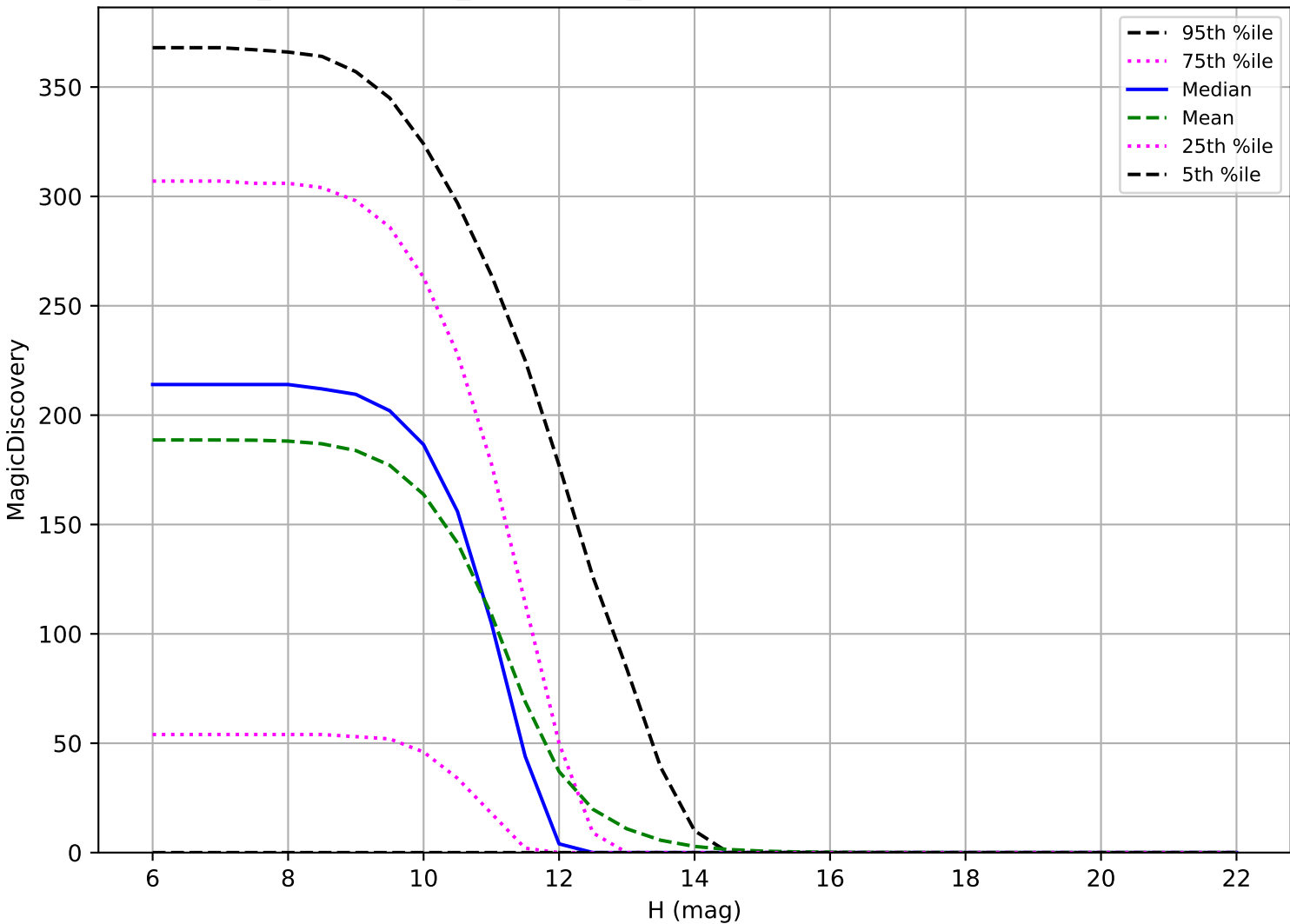
weather_cloudso2v3.4_10yrs: OCC_r20 6 detections in 60 nights detection loss
