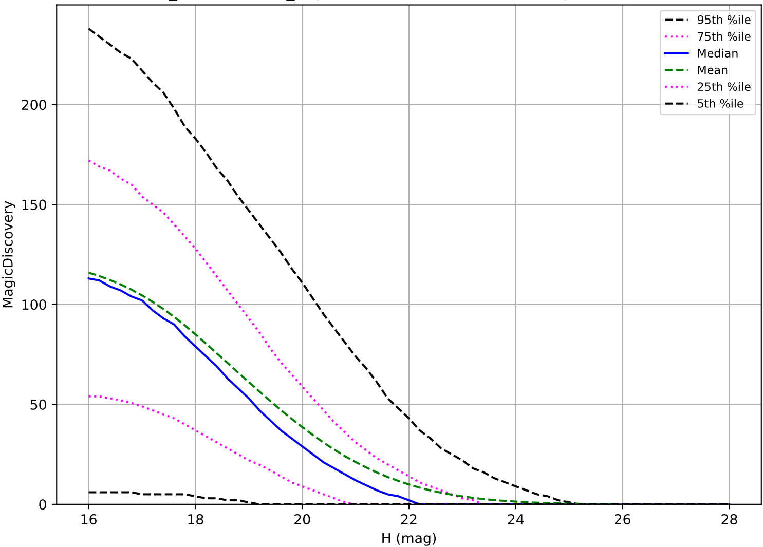
weather_cloudso2v3.4_10yrs: NEO 6 detections in 60 nights detection loss
