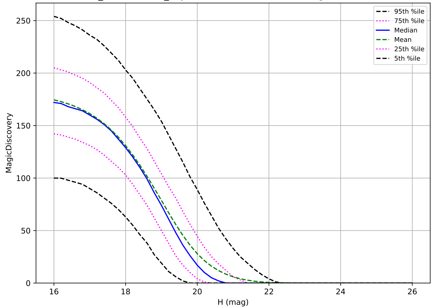
weather_cloudso2v3.4_10yrs: MBA 6 detections in 60 nights detection loss
