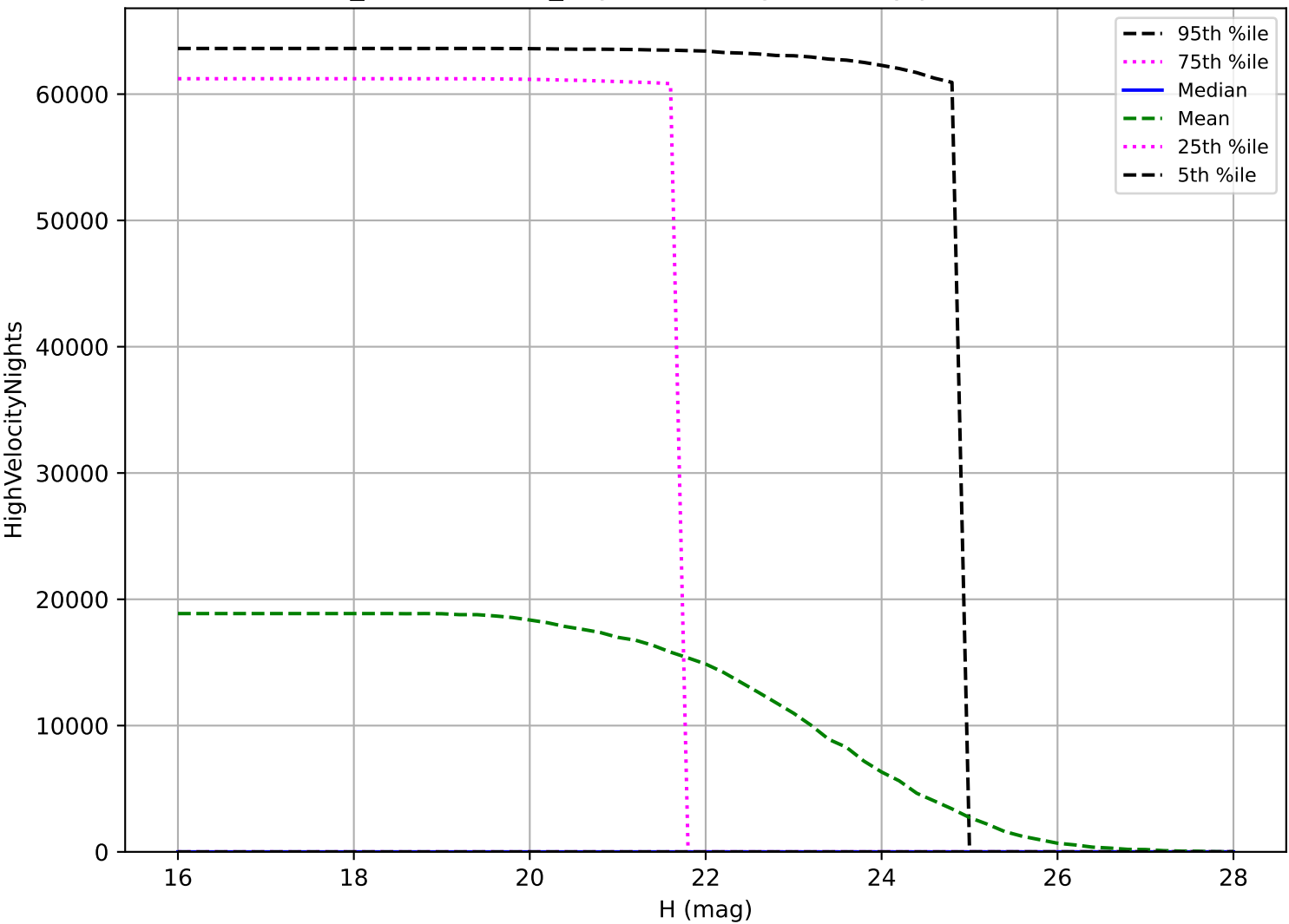
weather_cloudso2v3.4_10yrs: NEO High velocity pair detection loss
