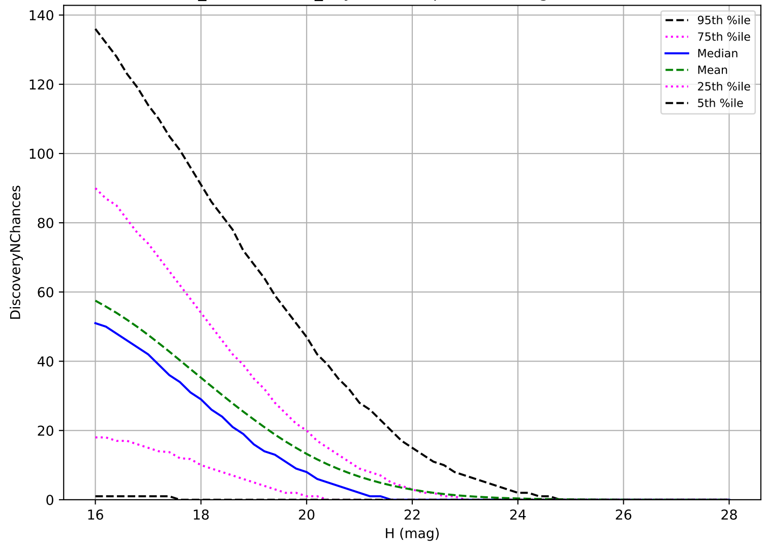
weather_cloudso2v3.4_10yrs: PHA 3 pairs in 15 nights detection loss
