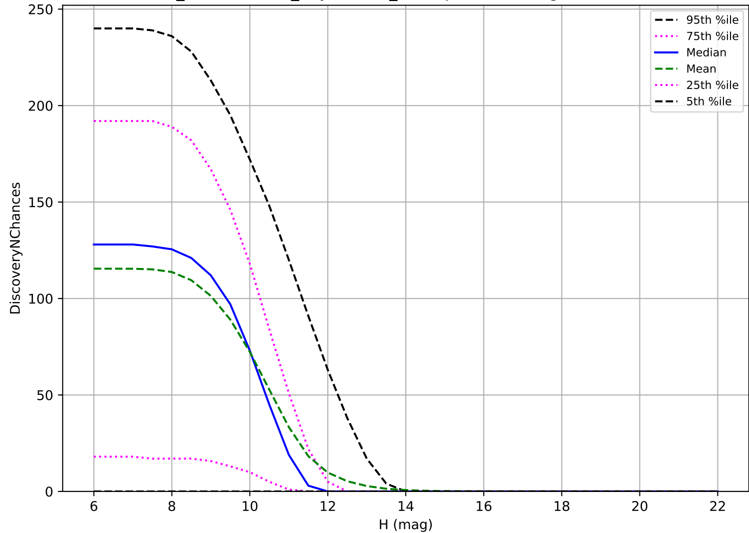
weather_cloudso2v3.4_10yrs: OCC_r20 3 pairs in 15 nights detection loss
