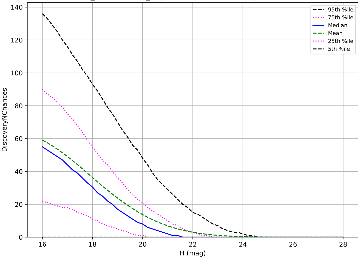
weather_cloudso2v3.4_10yrs: NEO 3 pairs in 15 nights detection loss
