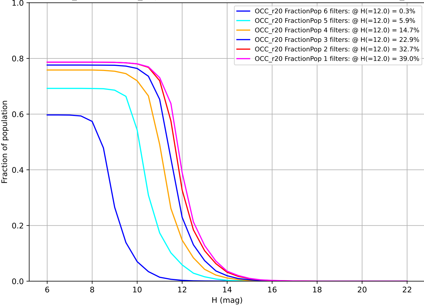
weather_cloudso2v3.4_10yrs: Fraction of population with colors in X filters OCC_r20
