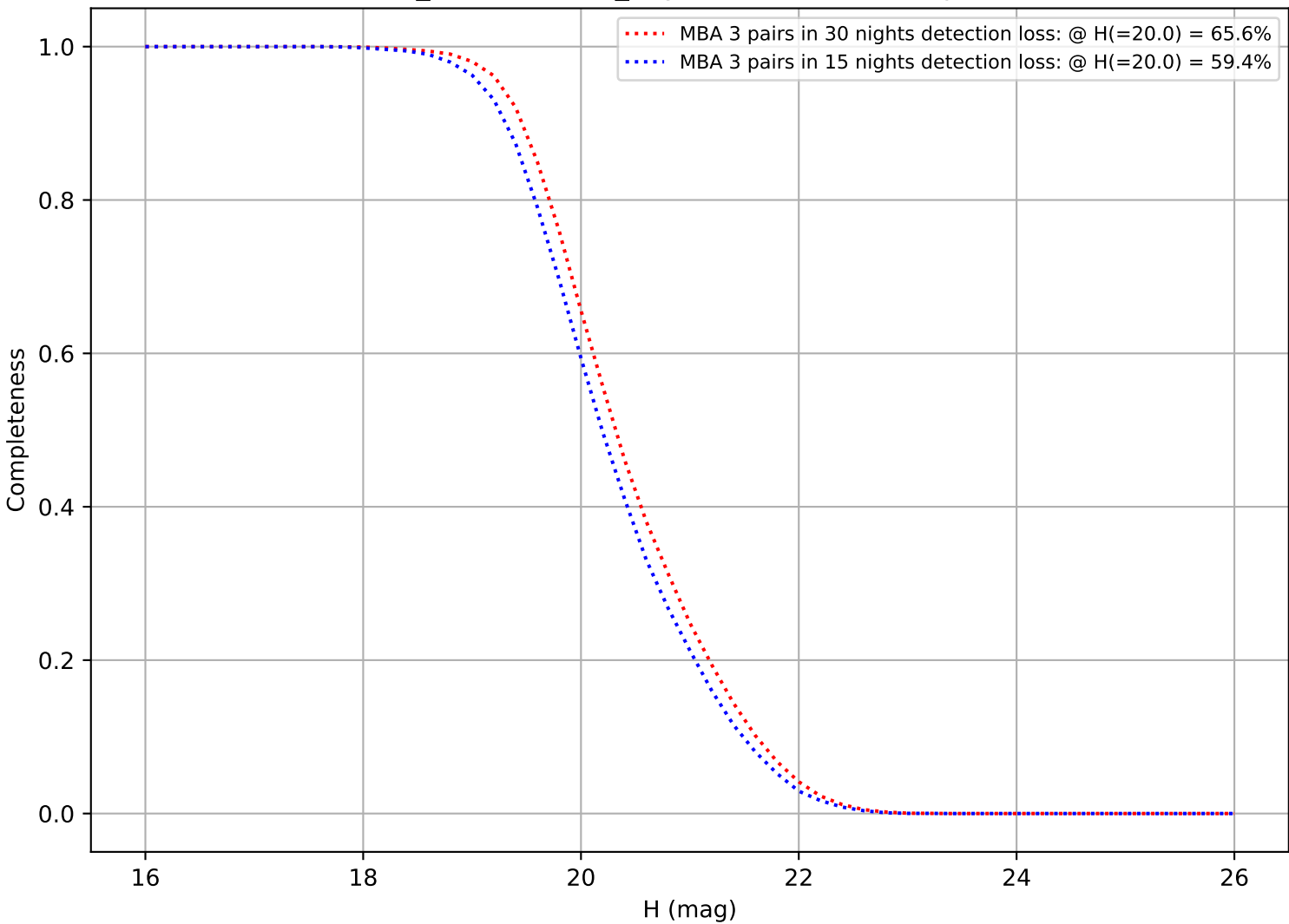
weather_cloudso2v3.4_10yrs: DifferentialCompleteness
