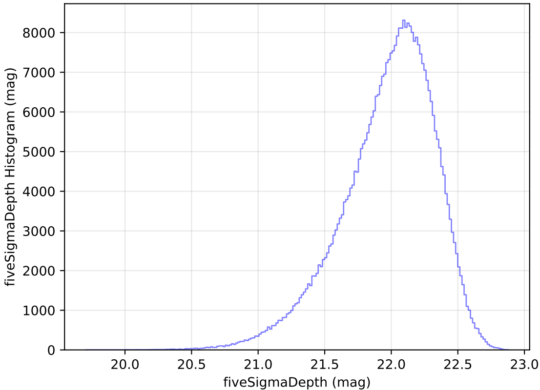
weather_cloudso2v3.4_10yrs y: fiveSigmaDepth Histogram
