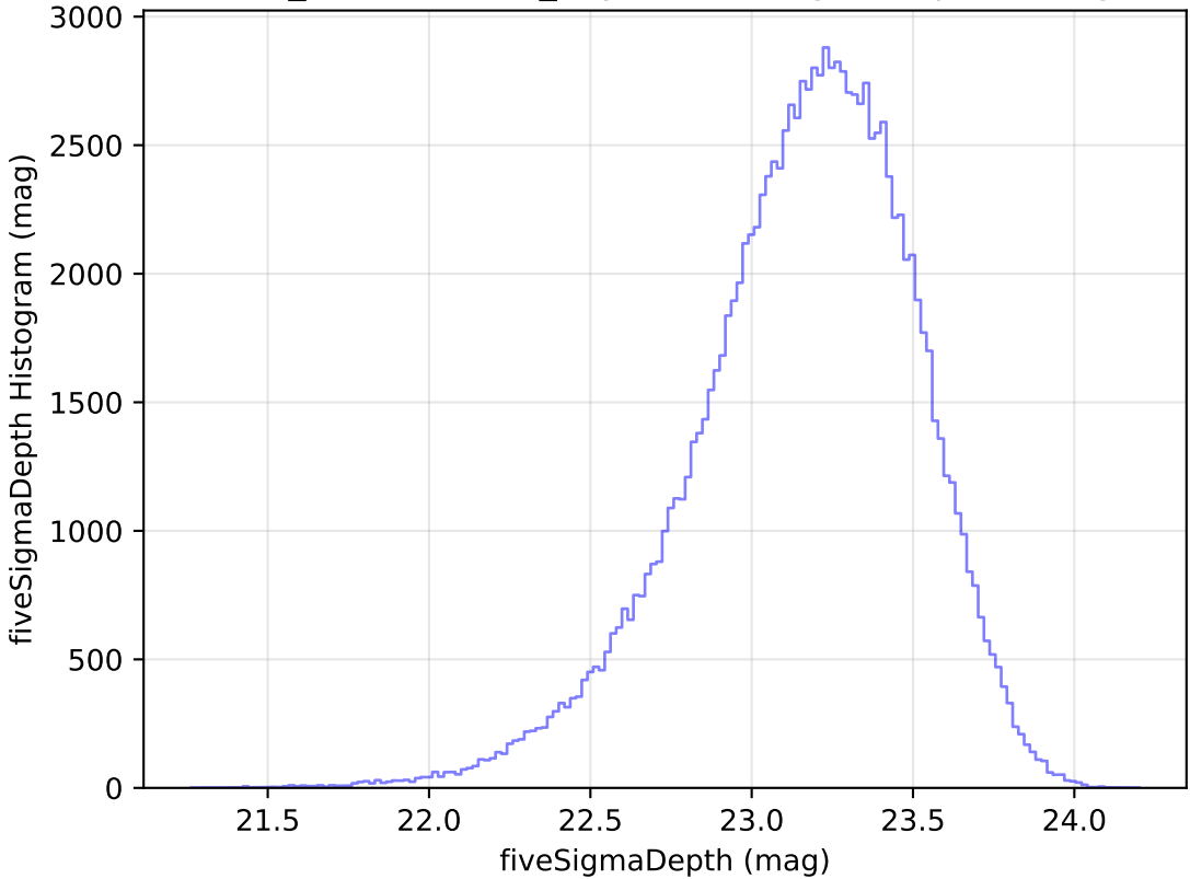
weather_cloudso2v3.4_10yrs u: fiveSigmaDepth Histogram
