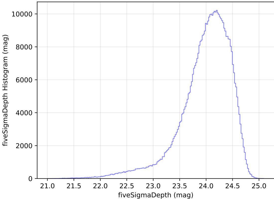
weather_cloudso2v3.4_10yrs r: fiveSigmaDepth Histogram
