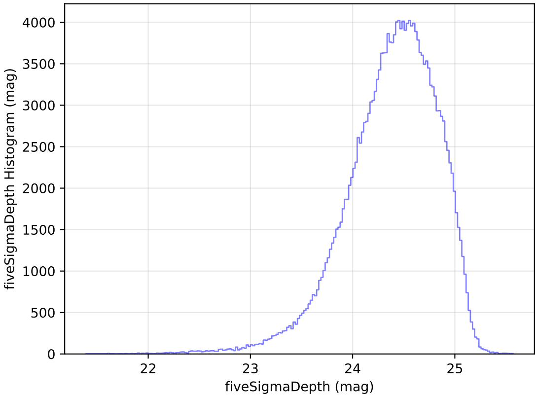
weather_cloudso2v3.4_10yrs g: fiveSigmaDepth Histogram
