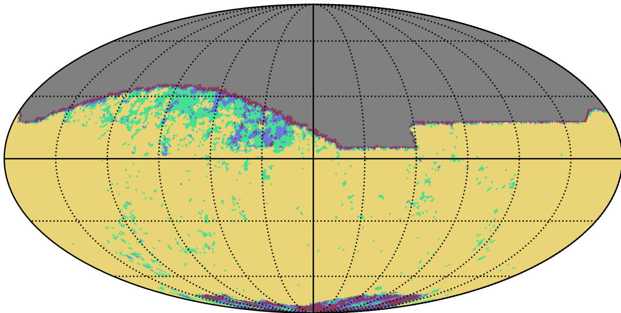
weather_cloudso2v3.4_10yrs z band: YearCoverage night
