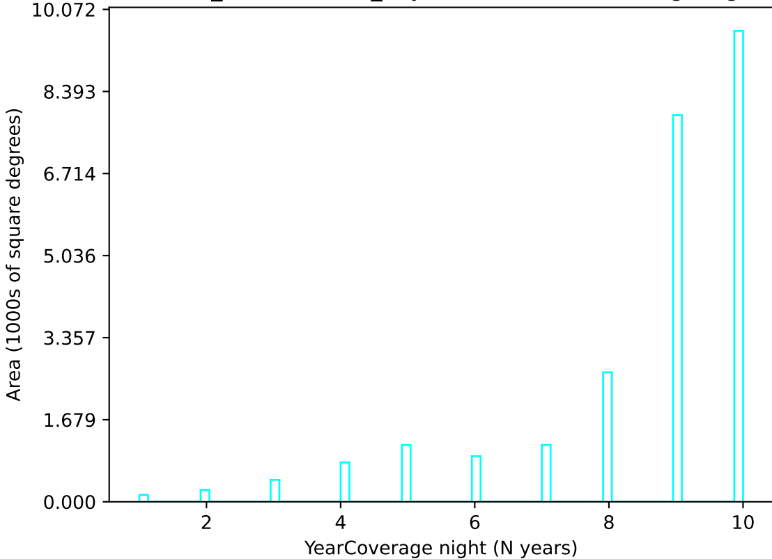
weather_cloudso2v3.4_10yrs u band: YearCoverage night
